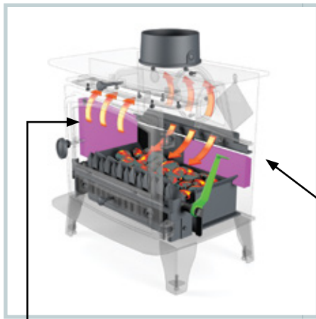
The Herald 'Internal Lining System' maximises the firebox temperature, ensuring complete combustion.
