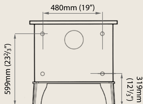
Wraparound Boiler Outlets
