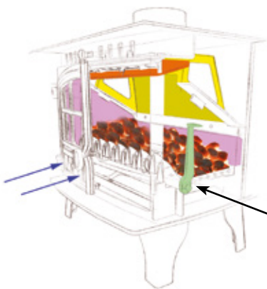
Grate in 'forward' open position for burning solid fuel
